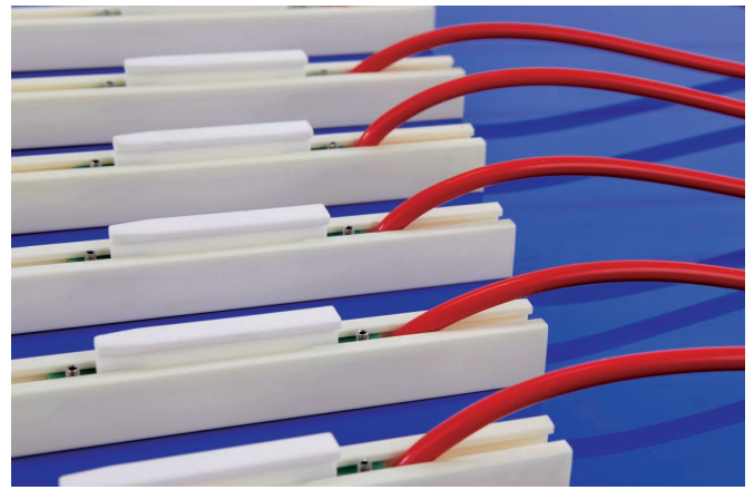
HV-Cable -exchangeable, in case of replacement or customization into existing systems. Ceramic clamps in ceramic rail.
